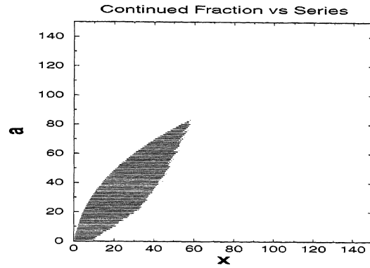
FIG. 2. Comparison between the evaluation of K_{i_a}(x) via continued fraction and via series expansion for a precision better than 10^{-9} . The x - a plane is scanned with point spacing \Delta a = 1 , \Delta x = 1 . The points where the coincidence between both approaches is at least of nine significant digits are shown.
