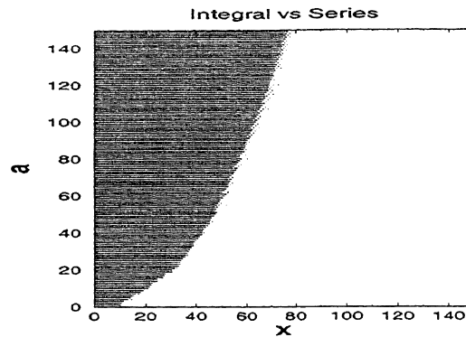
FIG. 5. Comparison between the evaluations via series expansion and via nonoscillating integral representation. The points of coincidence within a precision better than 10^{-9} are plotted.
